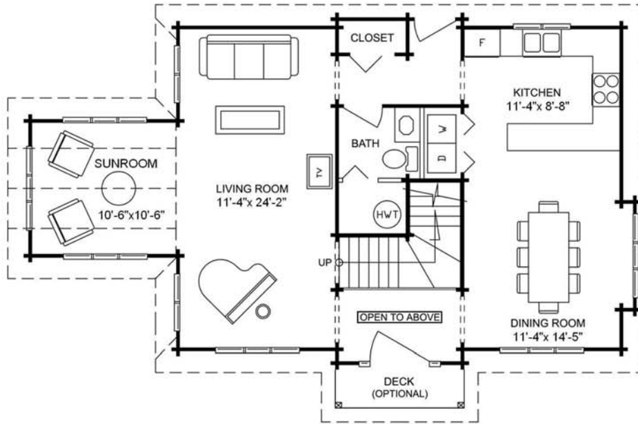
MAIN FLOOR PLAN 910 sq. ft. (84.52 sq. m.)
