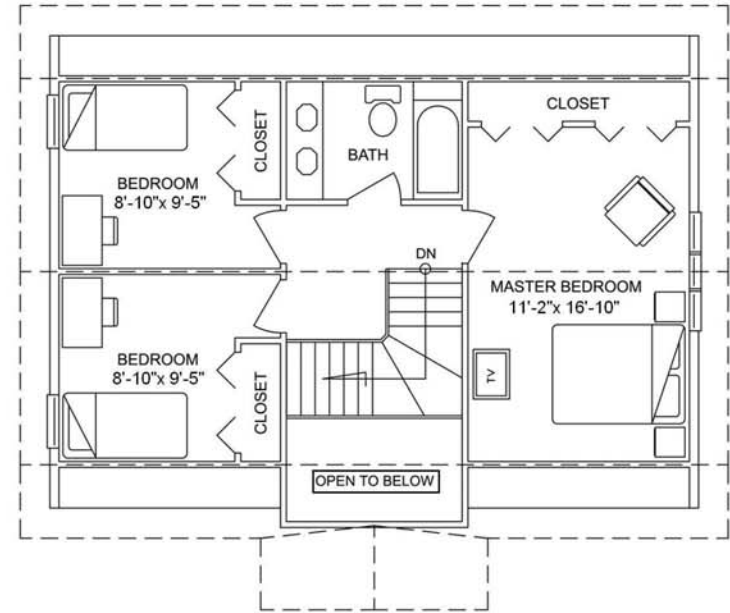
UPPER FLOOR PLAN 576 sq. ft. (53.48 sq. m.)
