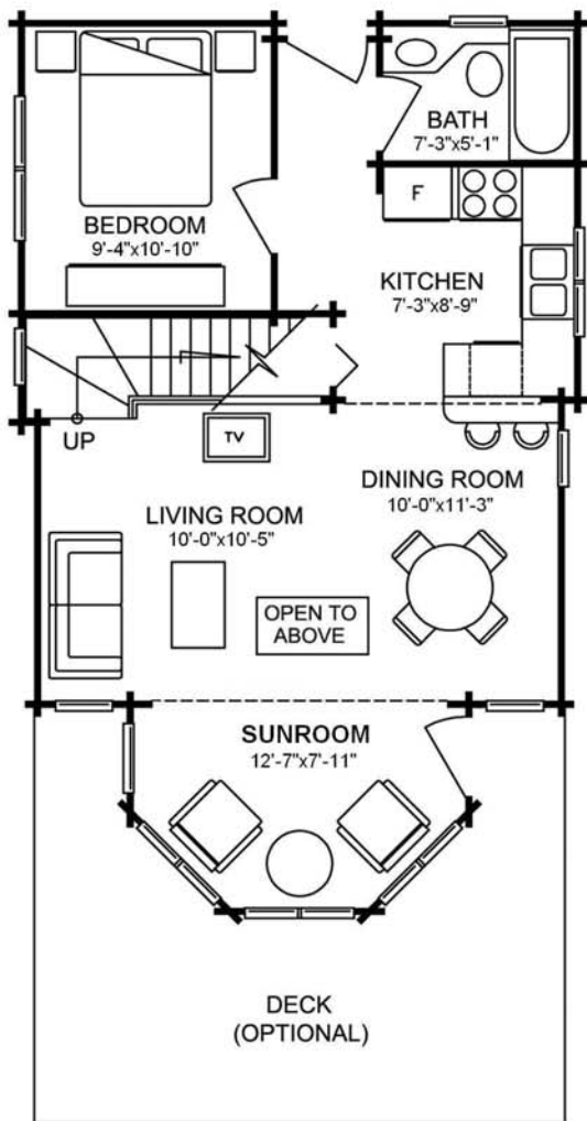
MAIN FLOOR PLAN 639 sq. ft. (59.39 sq. m.)
