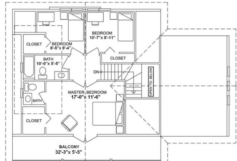
UPPER FLOOR PLAN 623 sq. ft. (57.86 sq. m.)
