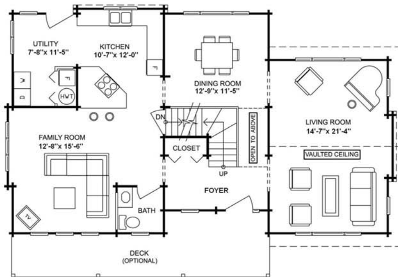
MAIN FLOOR PLAN 1203 sq. ft. (111.76 sq. m.)
