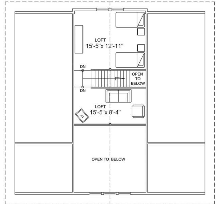
LOFT FLOOR PLAN 354 sq. ft. (32.87 sq. m.)
